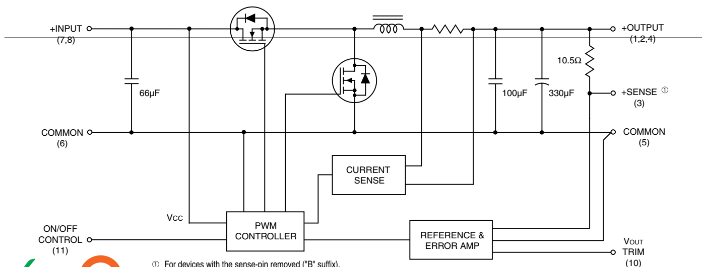
Figure 1. Simplified Schematic
