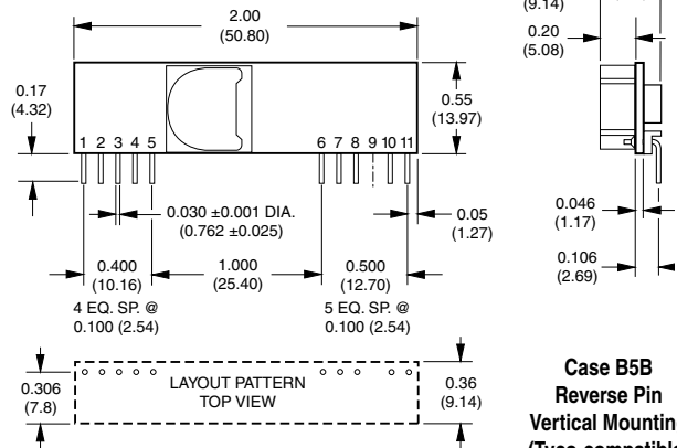
Case B5 Vertical Mounting (Standard)
